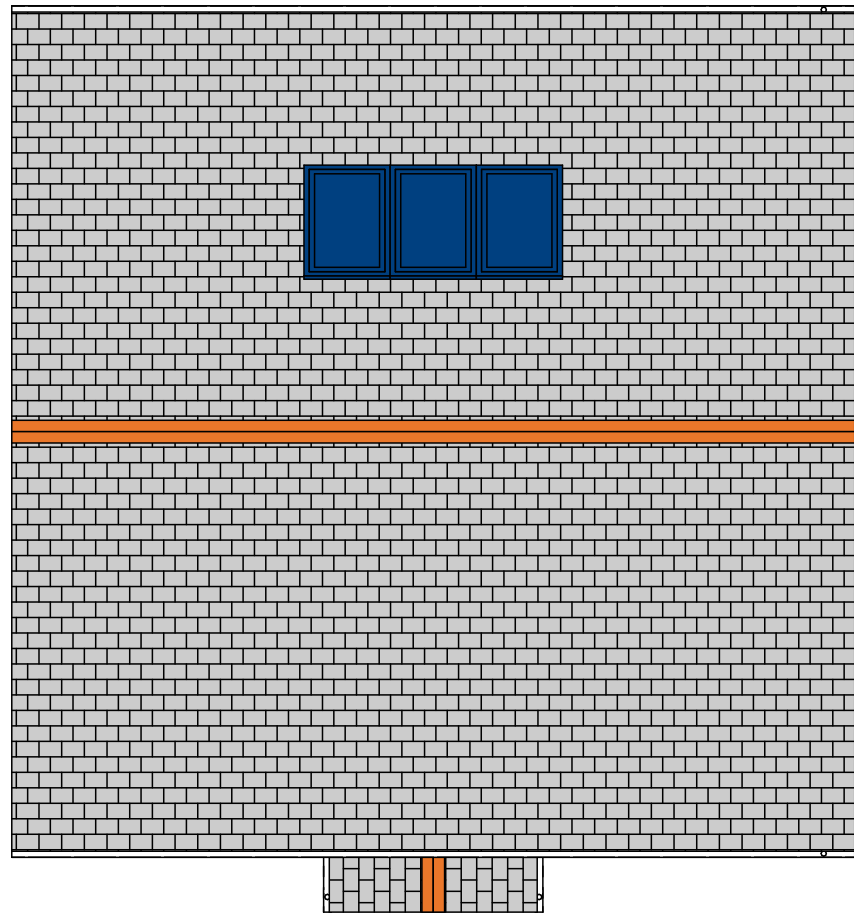
Roof Plan 1:100
